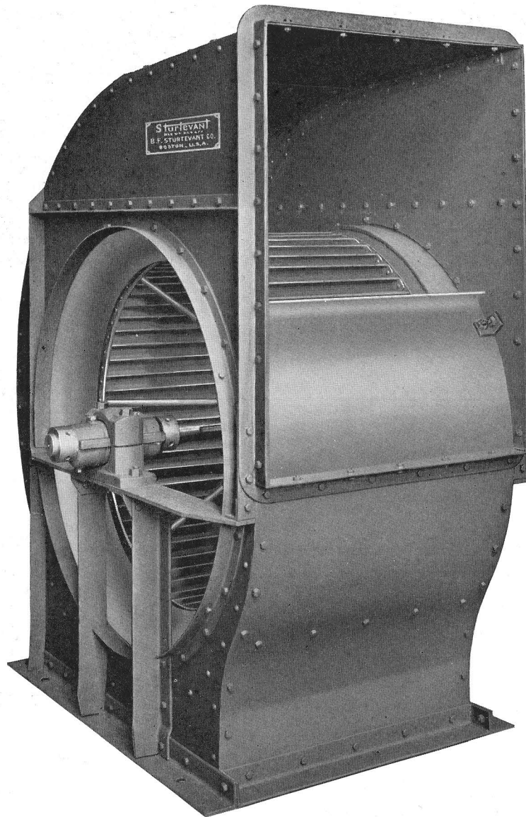
One of the larger size Design 6 Multivane Fans. This picture clearly shows the streamline inlet and location of cut off. This is an arrangement 3, single width, single inlet fan with bolted housing.
