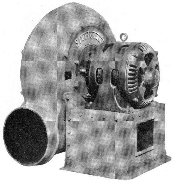
Design 3 Universal Monogram Fan, wheel overhung on motor shaft
